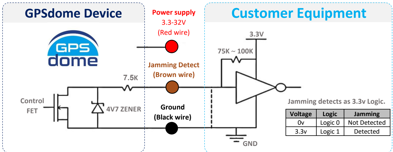
Figure 6 - Jamming Interference Detection Output Circuit
