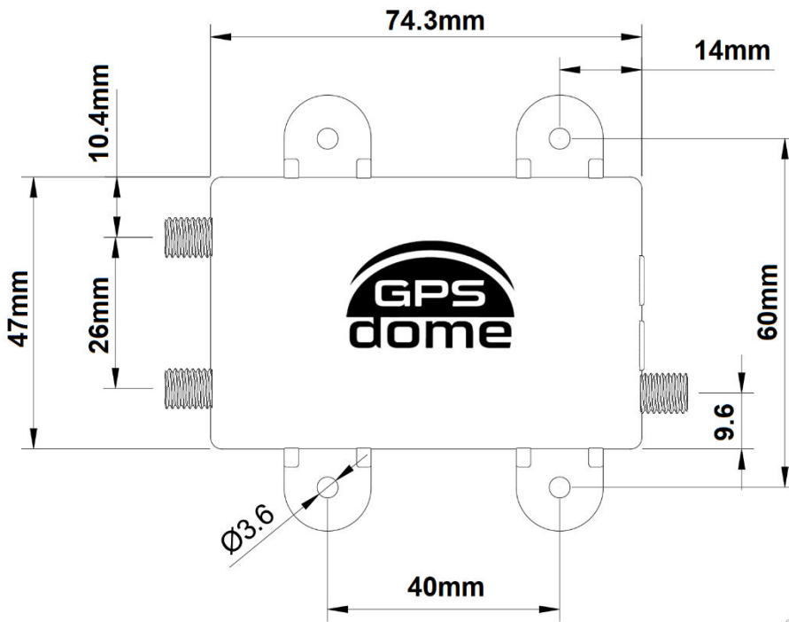
Figure 5 – GPSdome 1.03 - EPS – Product Dimensions
