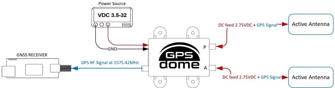
Figure 2 - GPS Receiver with GPSdome 1.03 - EPS Integrated
